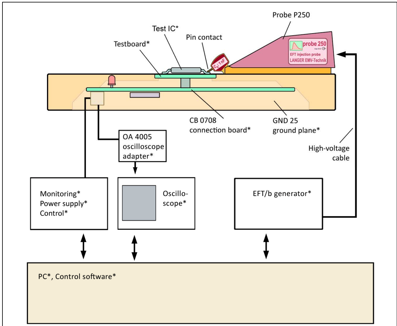
Figure 10: P250 probe in the test environment
